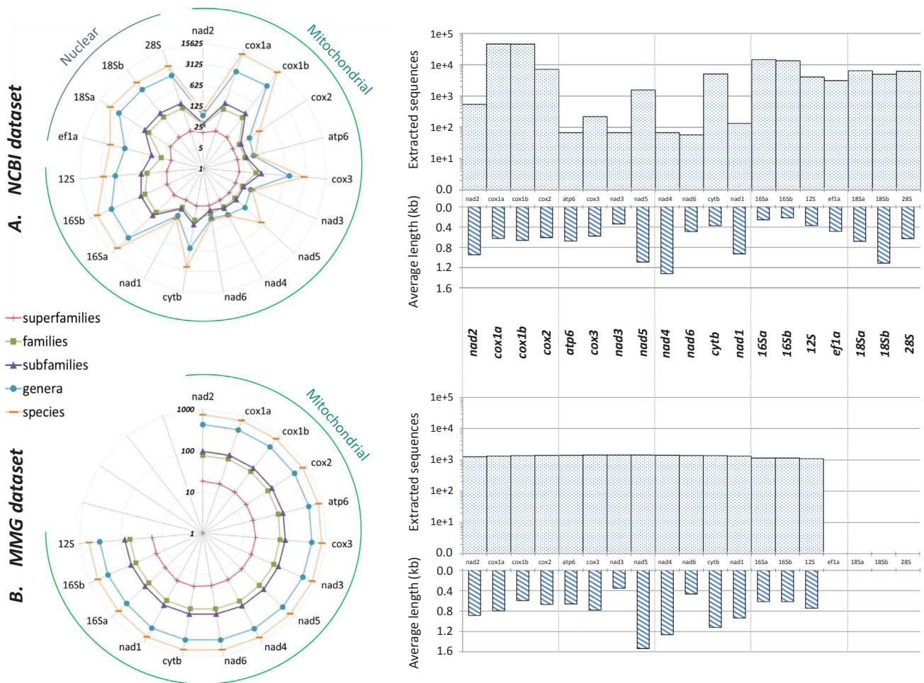
Fig. 2. Composition of the extracted sequence data. Loci statistics are reported for (A) the NCBI extraction (split in 15 mitochondrial and 4 nuclear loci) and (B) the MMG datasets (15 mitochondrial loci). Left radars illustrate the taxonomic evenness of the extraction, with one unit corresponding to one clade of the following taxonomic levels: species (orange dashes), genera (blue dots), subfamilies (purple triangles), families (green squares) and superfamilies (red crosses). On the right side, dotted histograms report the total number of entries retrieved for each locus (including multiple entries belonging to the same species) on a log scale, while dashed histograms reports the corresponding average sequence length.
