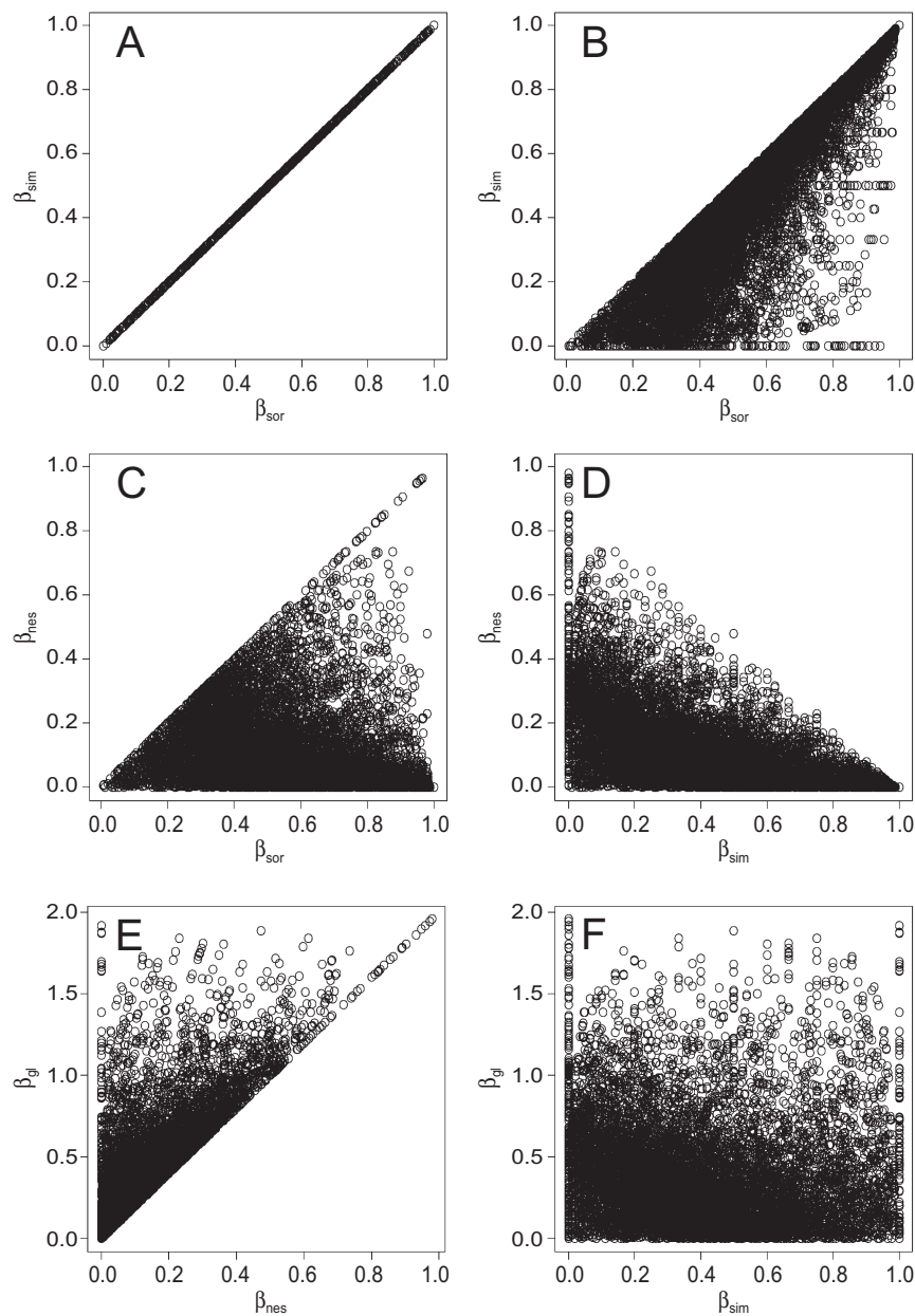
Figure 2 Relative performance of \beta_{\text{sor}} , \beta_{\text{sim}} , \beta_{\text{nes}} and \beta_{\text{gl}} under situations of equal (a) and unequal richness (b–f). Simulations were performed in R, taking random values of a , b and c matching components from uniform distributions between 1 and 100, where a is the number of species common to both sites, b is the number of species that occur in the first site but not in the second and c is the number of species that occur in the second site but not in the first. Under conditions of equal richness, b and c are always equal, so \beta_{\text{sor}} = \beta_{\text{sim}} and \beta_{\text{nes}} = 0 . Under conditions of unequal richness, b and c can take different values, so \beta_{\text{sim}} and \beta_{\text{nes}} randomly vary between \beta_{\text{sor}} and 0, but are mutually dependent as \beta_{\text{sor}} = \beta_{\text{sim}} + \beta_{\text{nes}} . The new measure \beta_{\text{nes}} is only slightly related to \beta_{\text{gl}} because the former accounts only for differences in composition due to nestedness, whereas the latter accounts for any difference in richness (as island D in Fig. 1, for example).
